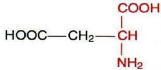
Acide aspartique (Asp, D)
