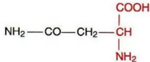
Asparagine (Asn, N)
