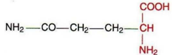
Glutamine (Gln, Q)
